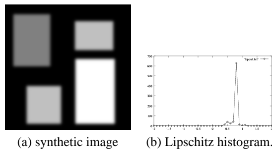
Figure 5. Blur estimation on synthetic image.
